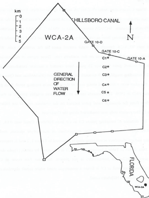
Figure 2. C-transect at the WCA-2A (borrowed from VYMAZAL et. al. 2000a). Similar transects were established also to the south from the gates 10-A and 10-D.
